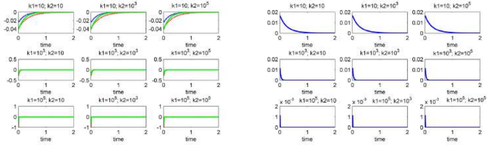
Figure 9: u^{\Delta t} (left) and \|y^{\Delta t}(\cdot)\| (right) for several values of k_1 and k_2 . The unstable equilibrium \theta is given by \{n_1, n_2, n_3\} = \{1, 0, 0(u)\} . The junctions used to control are 1, 2 and 3.
