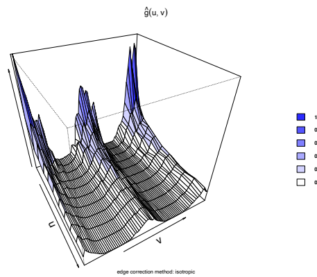
Figure 16: Estimated STPC function perspective plot.
