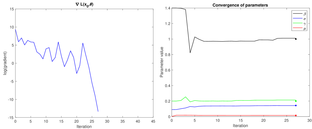
Figure 8: Left: plot of \log(\nabla L(\mathbf{x}_0, \theta)) against iteration obtained with the BFGS algorithm for 15% noisy data and observable variables ( E, I, R, D ). Right: convergence of \theta
