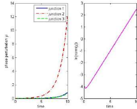
Figure 5: Solution \mathbf{y} = \delta\phi of (7) for the unstable equilibrium given by \{n_1, n_2, n_3\} = \{2, 1, 0(u)\} and \delta\theta = [1e-2, 1e-2, 1e-2] .
