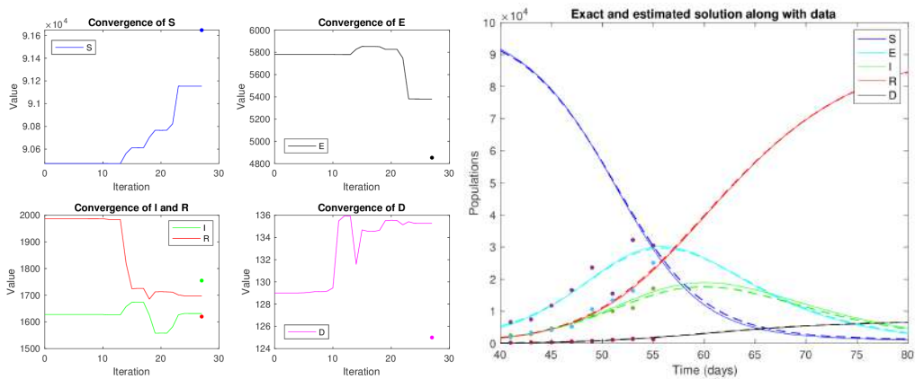
Figure 9: Left: convergence of \mathbf{x}_0 for 15% noisy data and observable variables ( E, I, R, D ). Right: dynamics of the true solution (continuous lines) and of the numerical solution (dashed lines).
