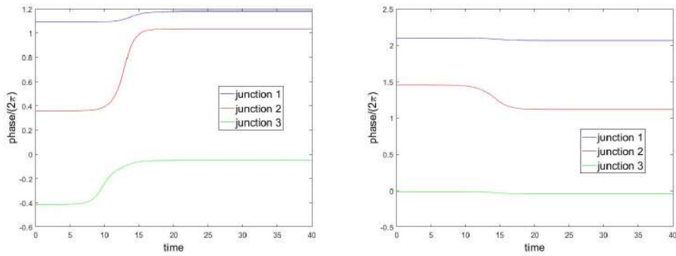
Figure 2: Evolution to state \{1, 1, 0(s)\} (left), \{2, 1, 0(s)\} (right) from an approximation to the unstable equilibrium \{1, 0, 0(u)\} (left), \{2, 1, 0(u)\} (right).
